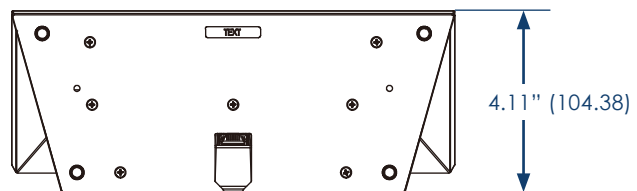
MT-1002 (Bottom View)
